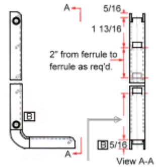
Type 7 - Stamped Ferrule Option
