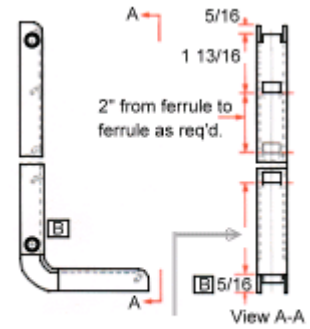
Type 7 - Stamped Ferrule Option
