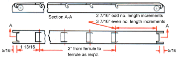
Type 8 - Stamped Ferrule Option
