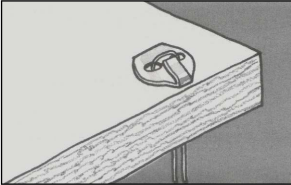
1. INSTALL LACING HOOK WITH TIE WIRE.
