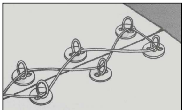
3. SECURE INSULATION BY LACING THRU RINGS.
